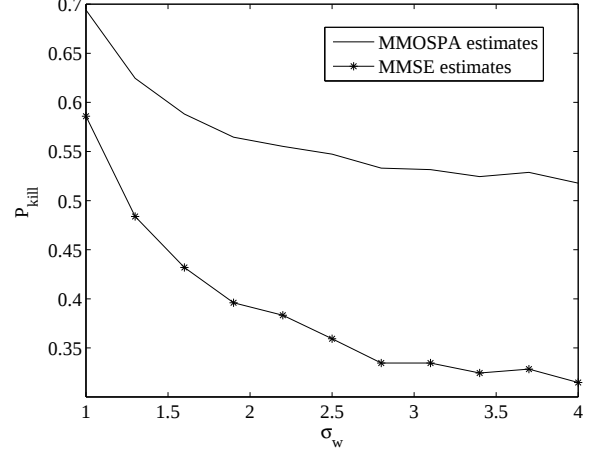
Figure 5: Kill probability P_{kill}(\hat{\mathbf{x}}, \epsilon) for the MMOSPA and the MMSE estimators, respectively. Here we used 1000 Monte Carlo trials and \epsilon = 1 .
